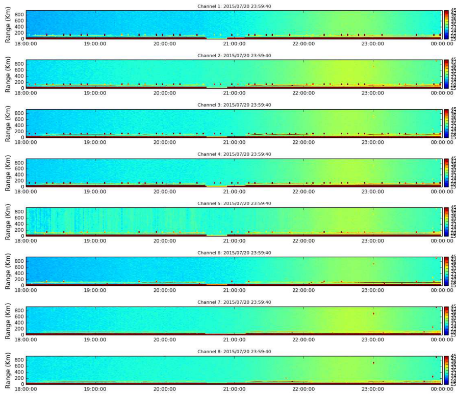
Figure 2. RTI IMAGING 2015-07-20 18:00-24:00.
