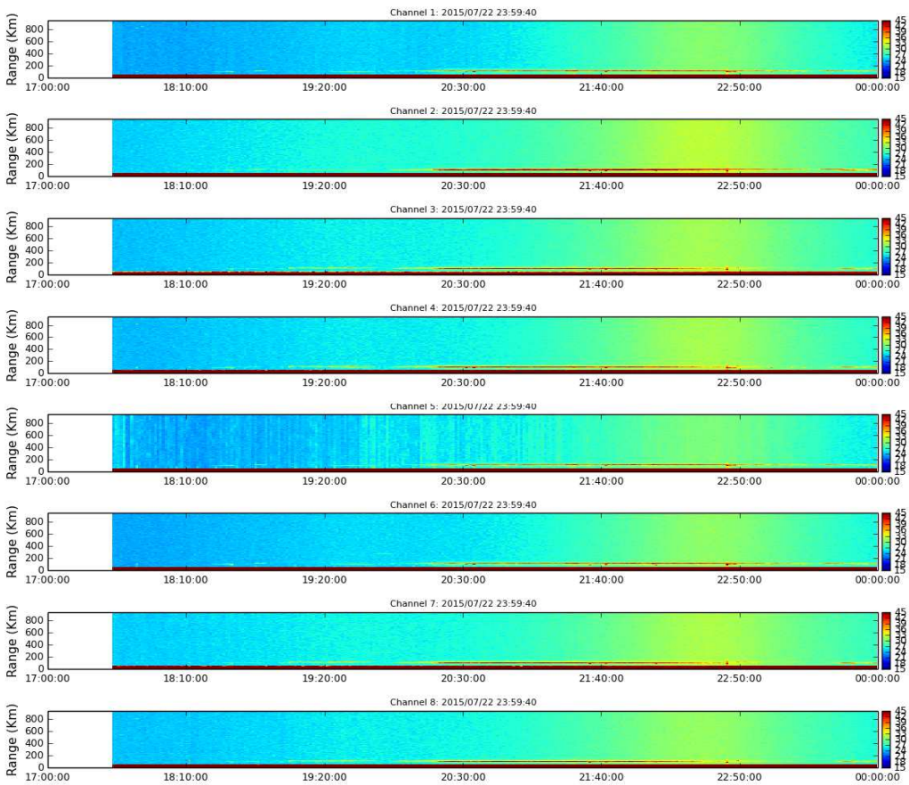
Figure 11. Rti IMAGING 2015-07-22 18:00-24:00.
