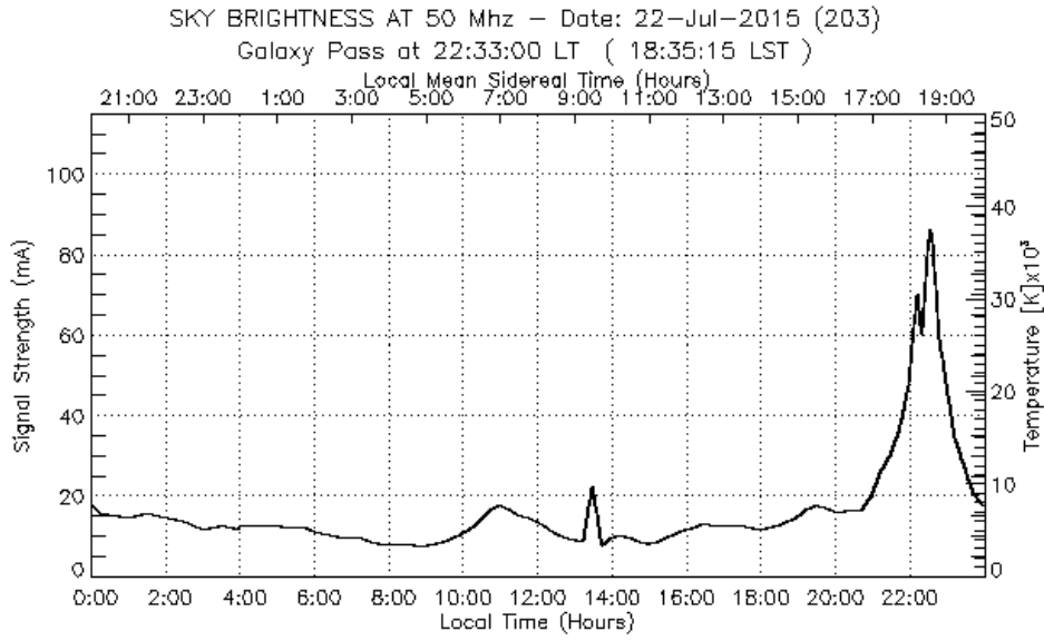
Figure 17. Sky noise.
