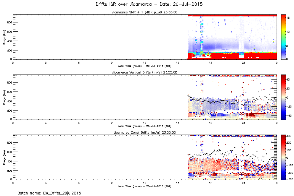
Figure 3. Drifts 2015-07-20.
