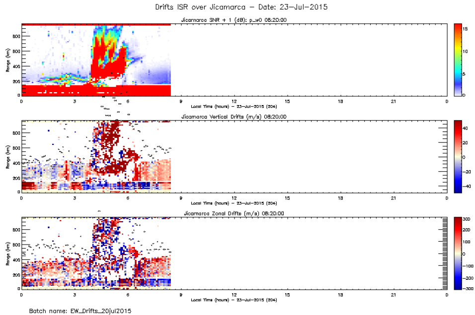
Figure 16. Drifts 2015-07-23.
