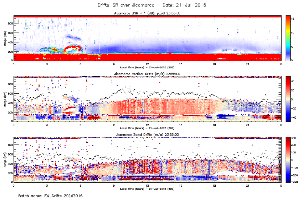
Figure 8. Drifts 2015-07-21.
