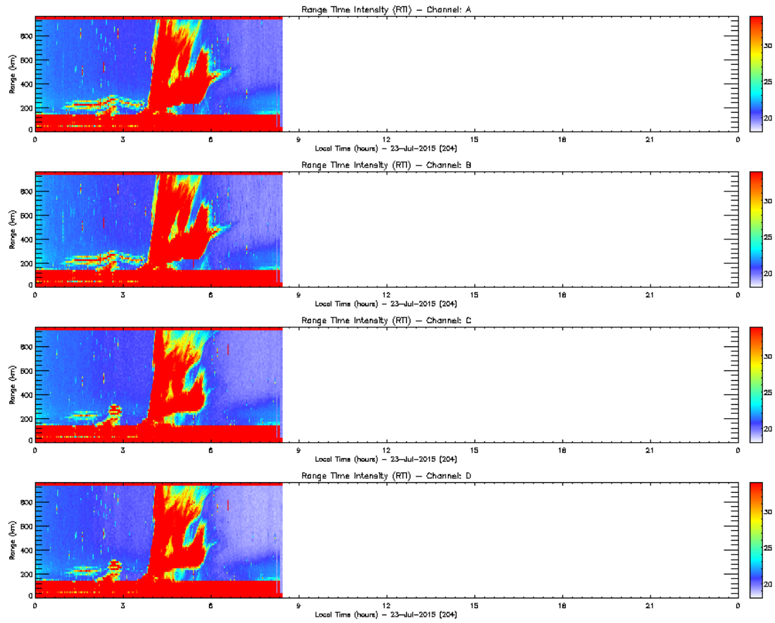
Figure 13. Rti EW_DRIFT 2015-07-23
