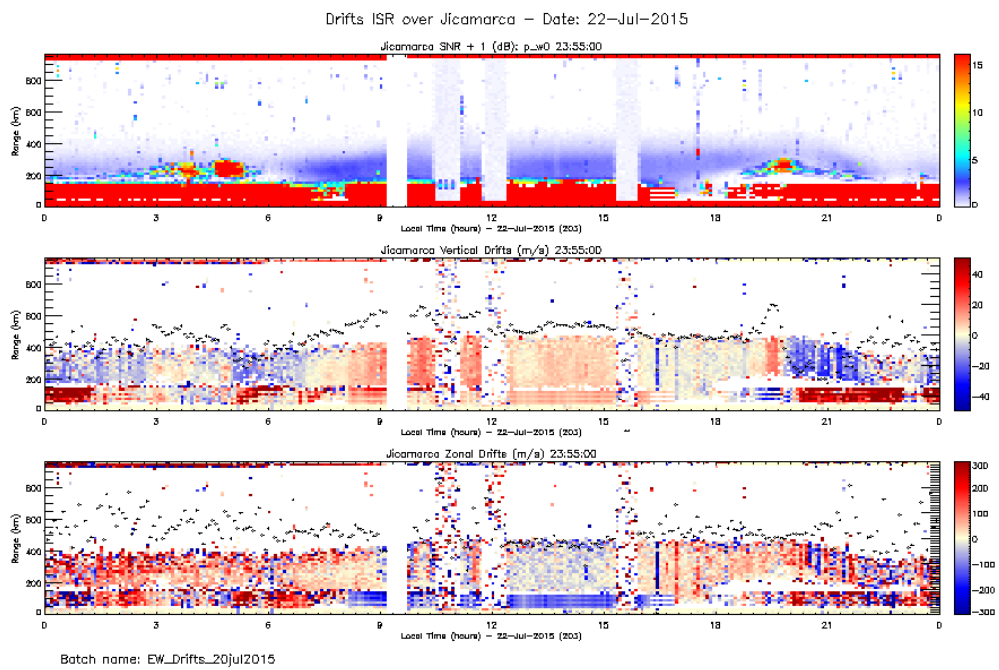
Figure 12. Drifts 2015-07-22
