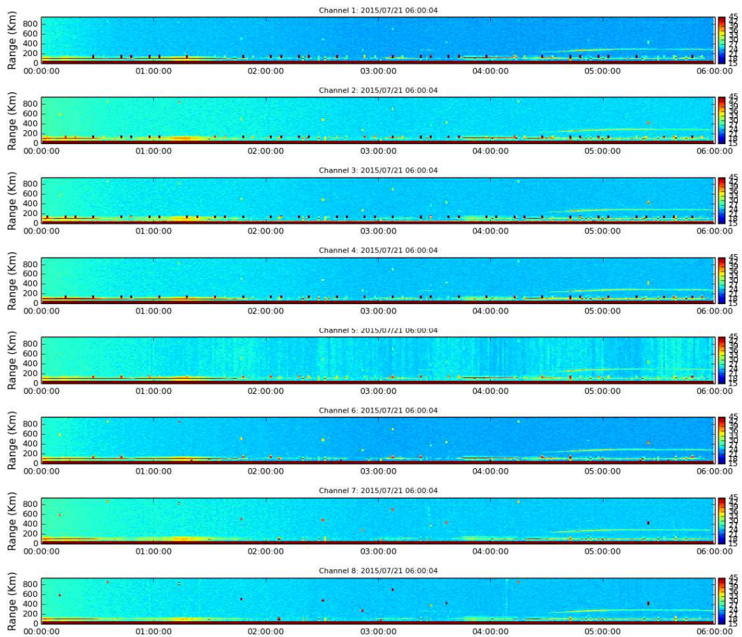
Figure 5. Rti FARADAY 2015-07-21
