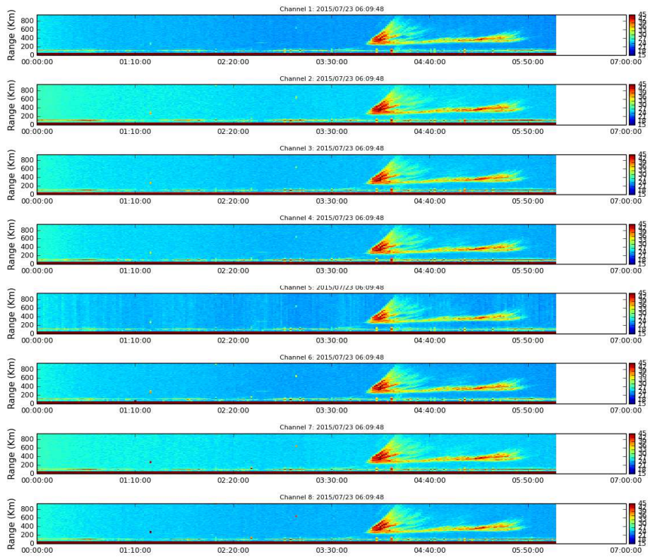
Figure 15. Rti IMAGING 2015-07-23 00:00-06:00.
