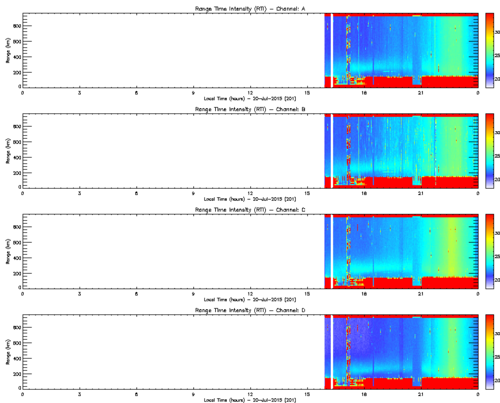
Figure 1.Rti EW_DRIFT 2015-07-20.
