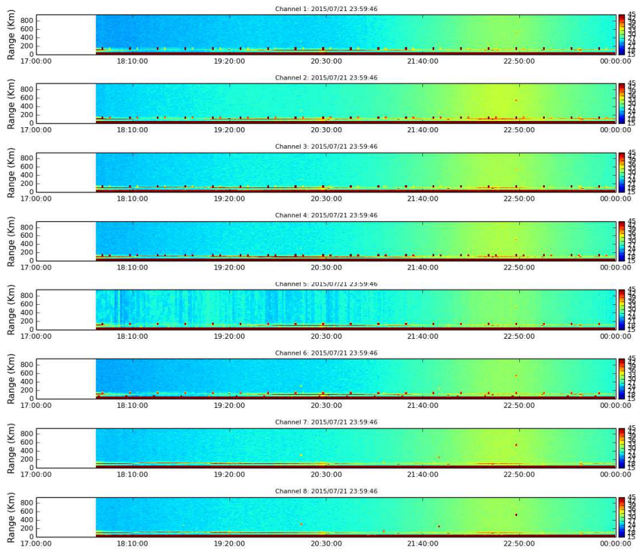
Figure 7. Rti IMAGING 2015-07-21 18:00-24:00.
