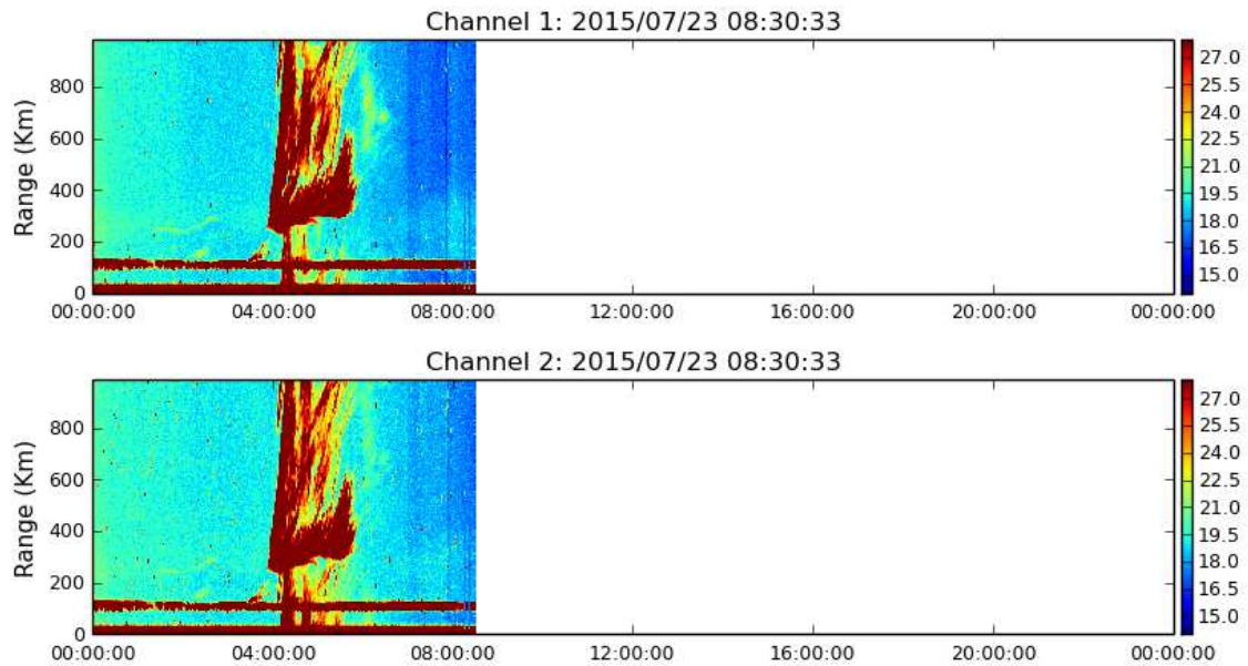
Figure 13. Rti EW_DRIFT 2015-07-23
