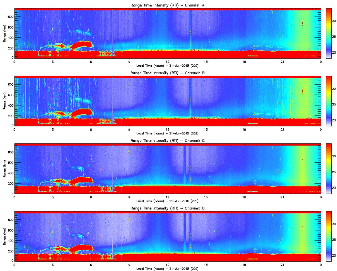
Figure 4. Rti EW_DRIFT 2015-07-21.
