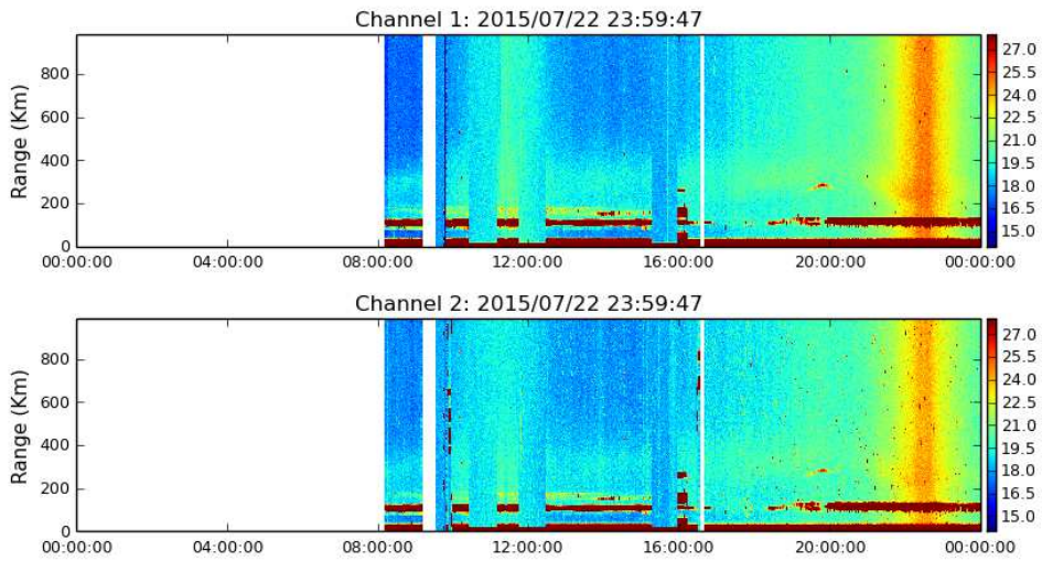
Figure 10. Rti FARADAY 2015-07-22.
