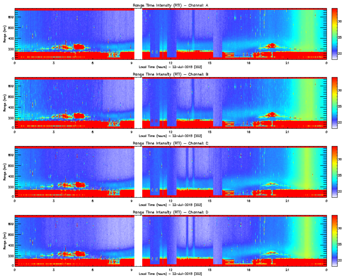
Figure 9. Rti EW_DRIFT 2015-07-22.
