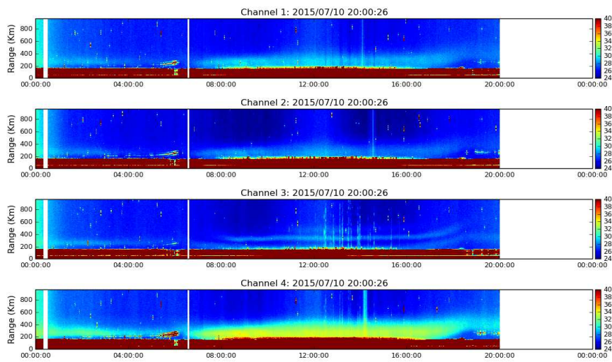
Figure 11. Rti ISR 2015-07-10.
