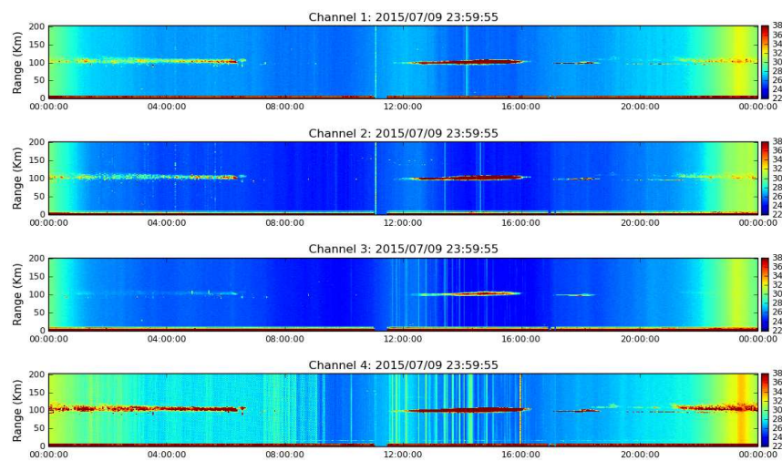
Figure 9. Rti EEJ 2015-07-09.
