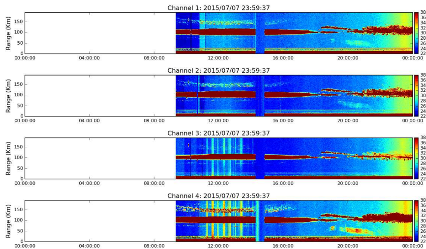
Figure 1.Rti MST 2015-07-07.
