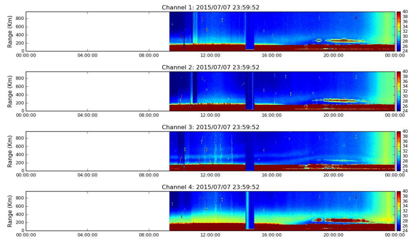
Figure 2. Rti ISR 2015-07-07.
