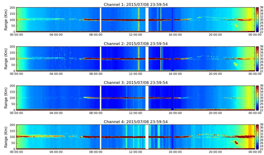
Figure 6. Rti EEJ 2015-07-08.
