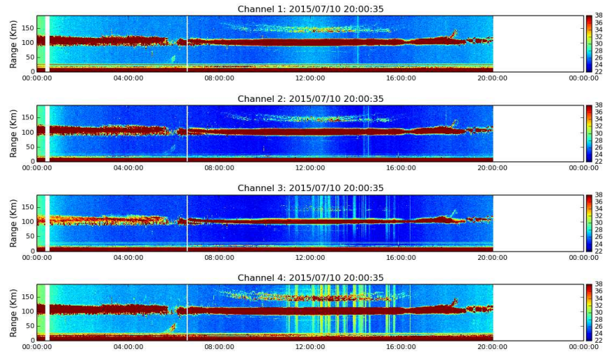
Figure 10. Rti MST 2015-07-10.
