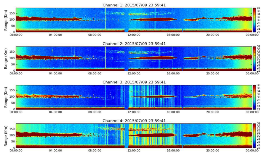
Figure 7. Rti MST 2015-07-09.
