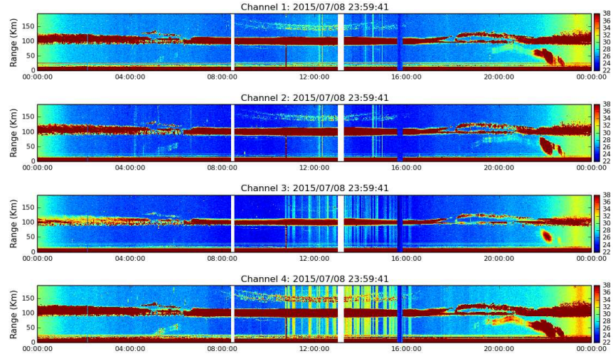
Figure 4. Rti MST 2015-07-08.
