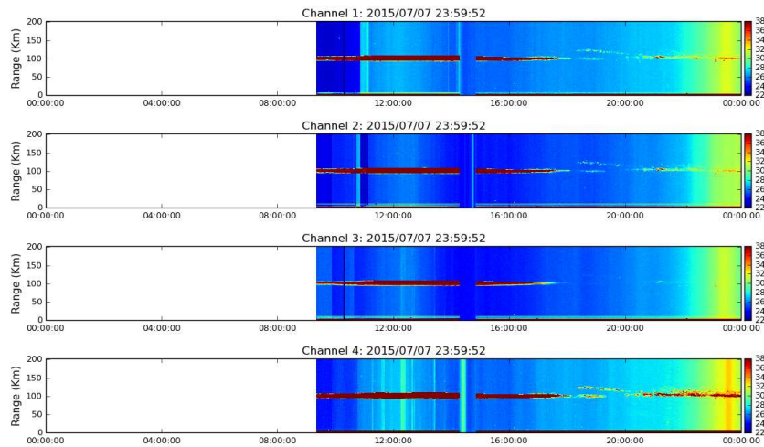
Figure 3. RTI EEJ 2015-07-07.
