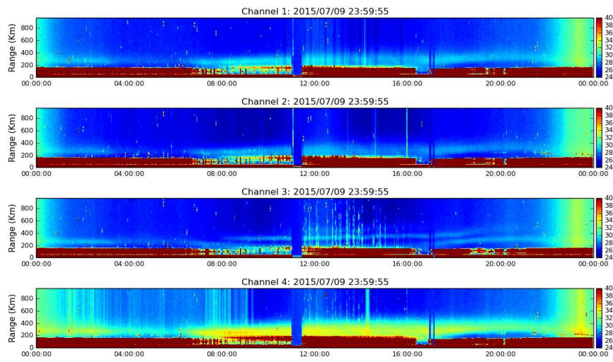
Figure 8. Rti ISR 2015-07-09.
