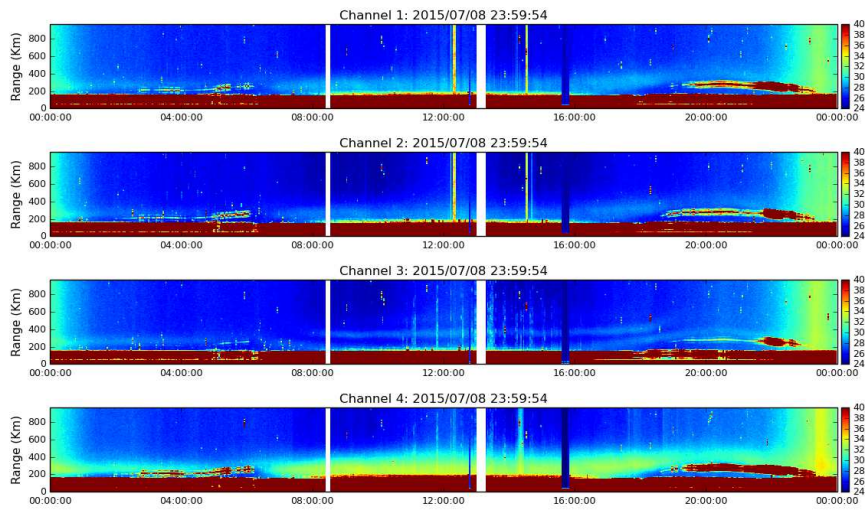
Figure 4. Rti MST 2015-07-08.
