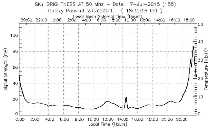
Figure 13. Sky noise.
