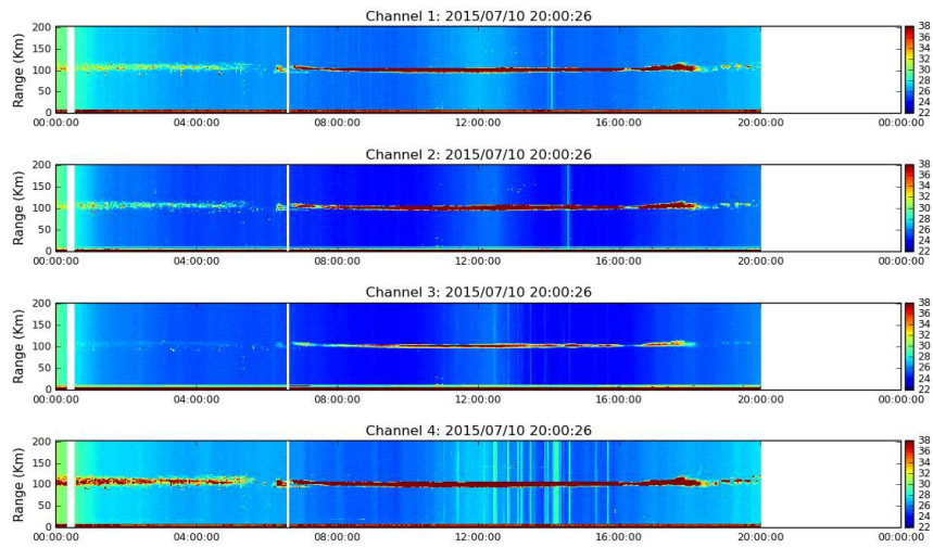
Figure 12. Rti EEJ 2015-07-10.
