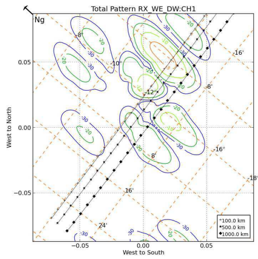
Figure 17. Antennas pattern, Ch 1 and Ch 2.
