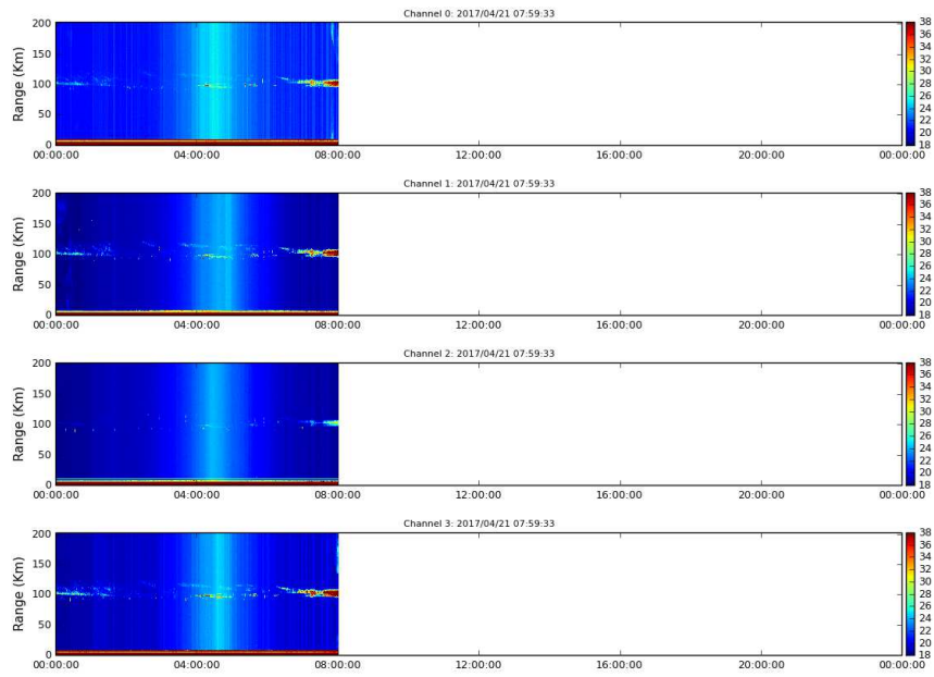
Figure 15. Rti EEJ 2017-04-21.
