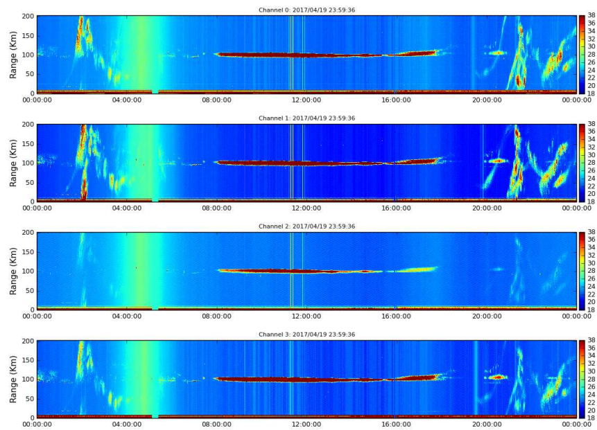
Figure 9. Rti EEJ 2017-04-19.
