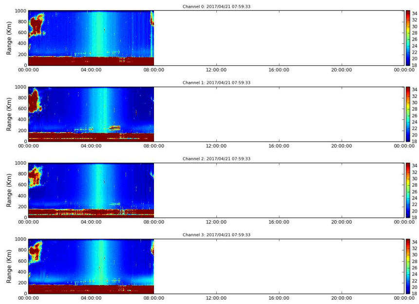
Figure 14. Rti ISR 2017-04-21.
