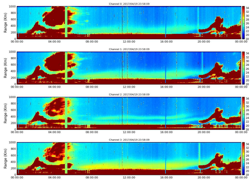
Figure 8. Rti ISR 2017-04-19.
