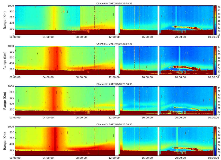
Figure 5. Rti ISR 2017-04-18.
