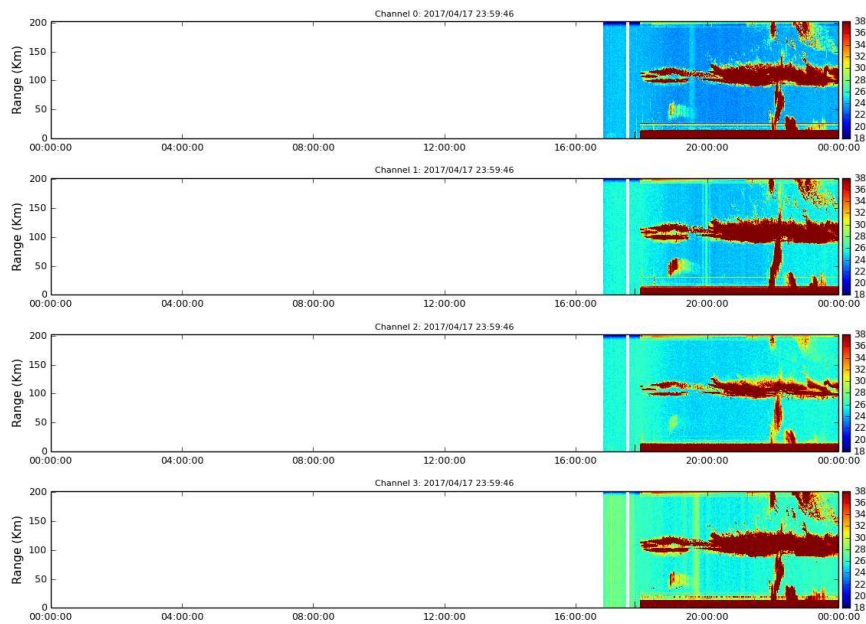
Figure 1.Rti MST 2017-04-17.
