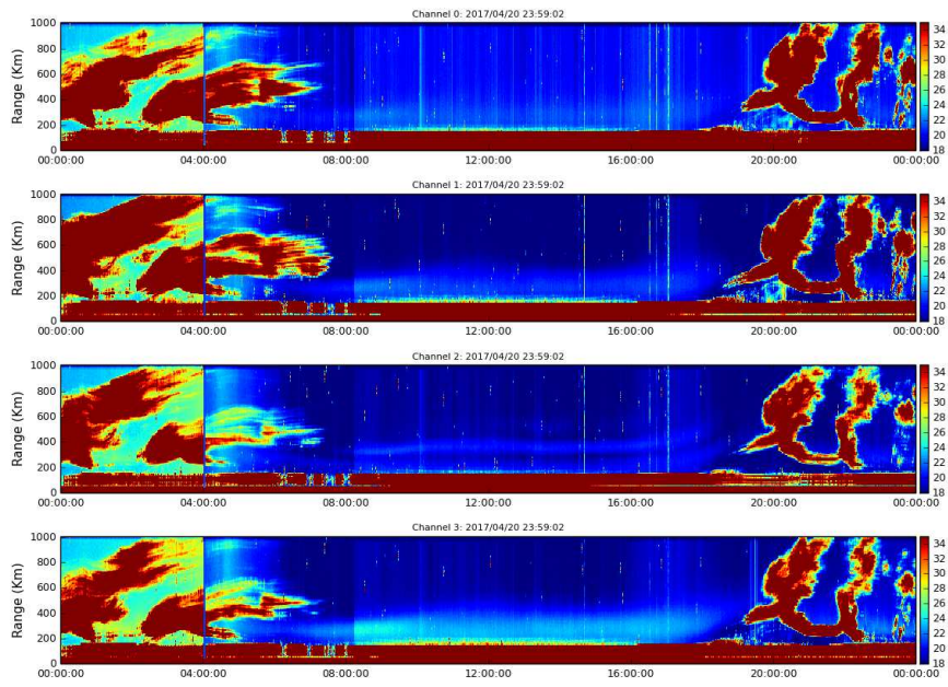
Figure 11. Rti ISR 2017-04-20.
