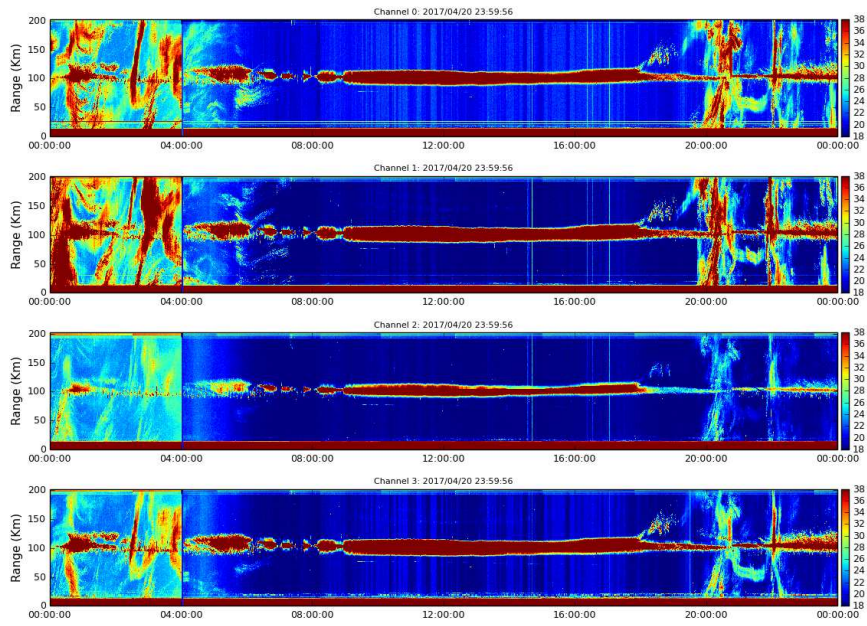
Figure 10. Rti MST 2017-04-20.
