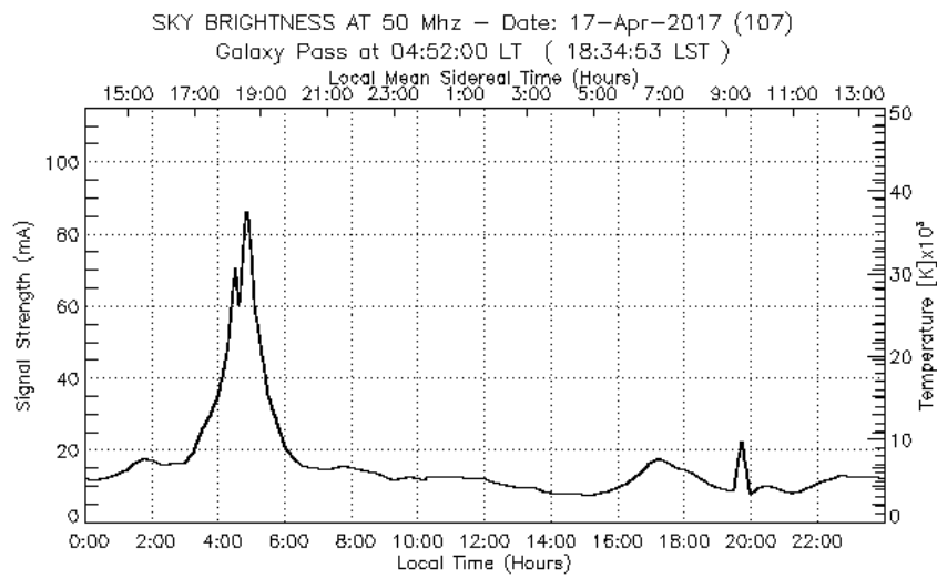
Figure 16. Sky noise.
