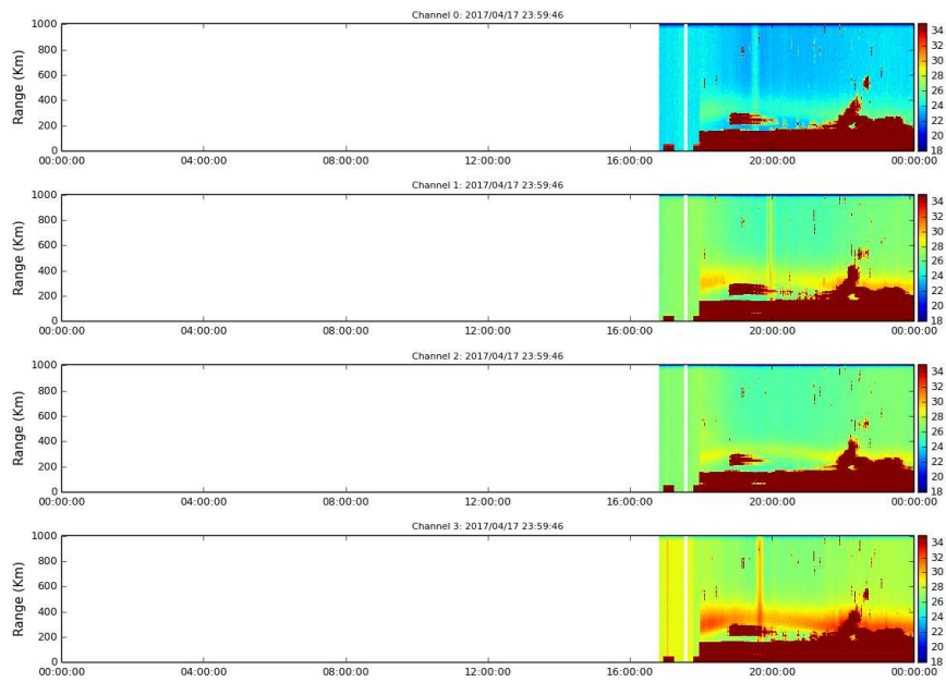
Figure 2. Rti ISR 2017-04-17.
