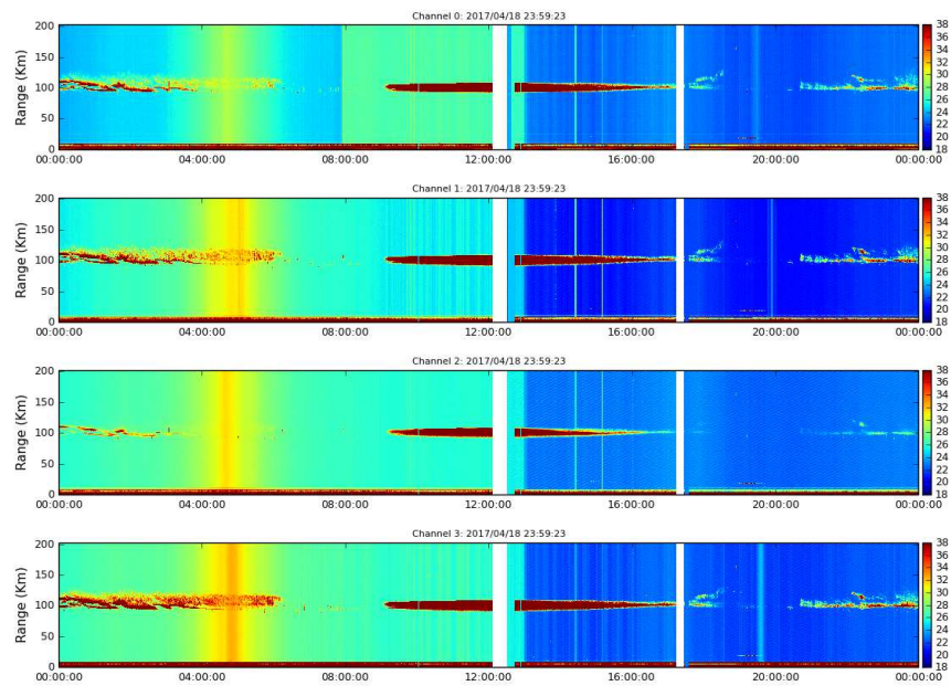
Figure 6. Rti EEJ 2017-04-18.
