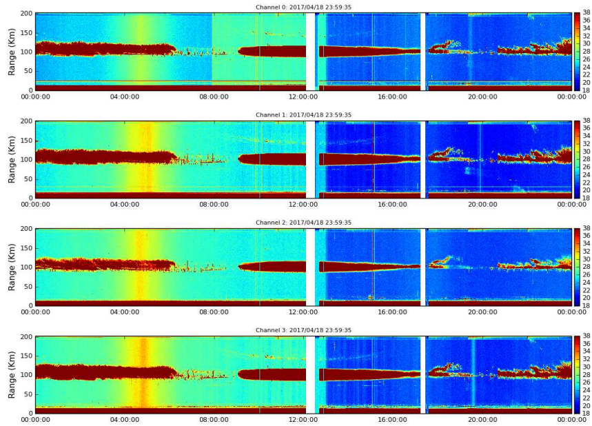
Figure 4. Rti MST 2017-04-18.
