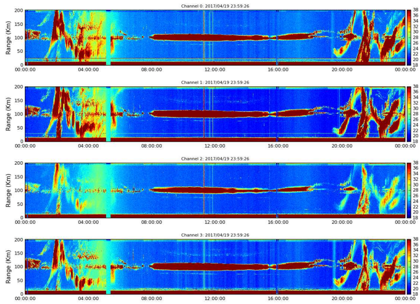
Figure 7. Rti MST 2017-04-19.
