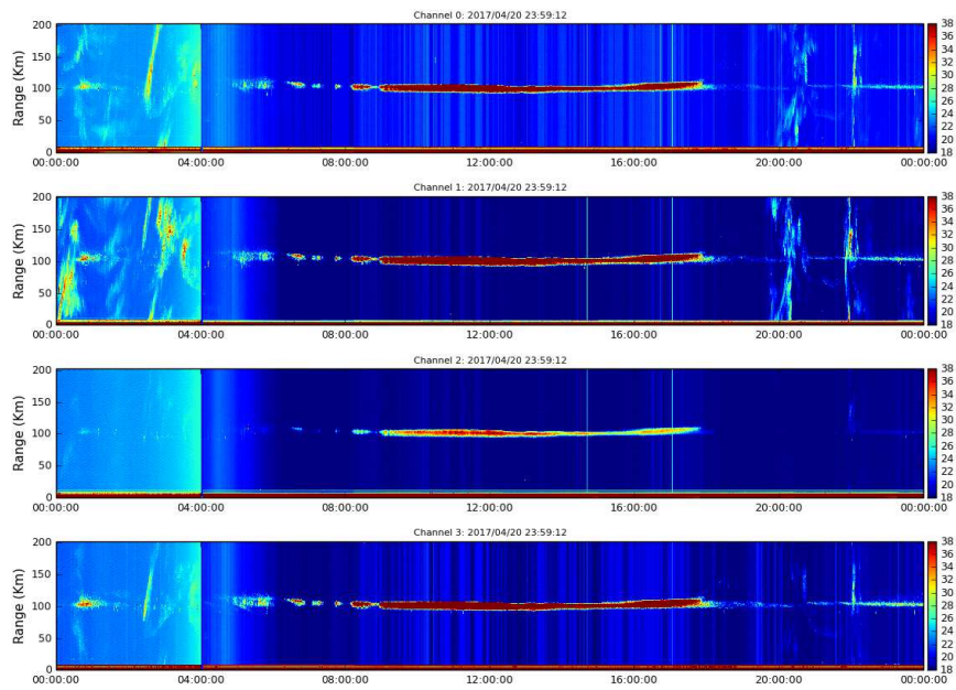
Figure 12. Rti EEJ 2017-04-20.
