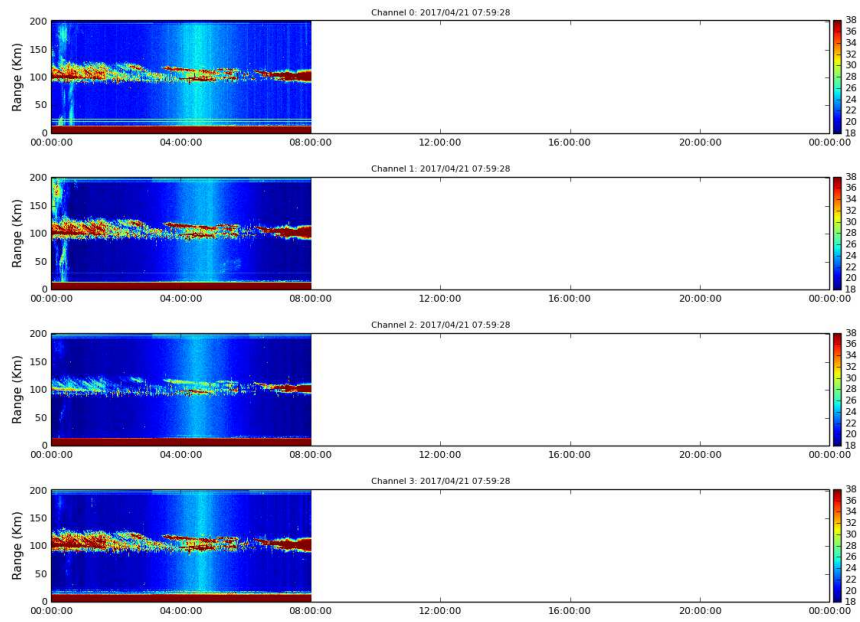
Figure 13. Rti MST 2017-04-21.
