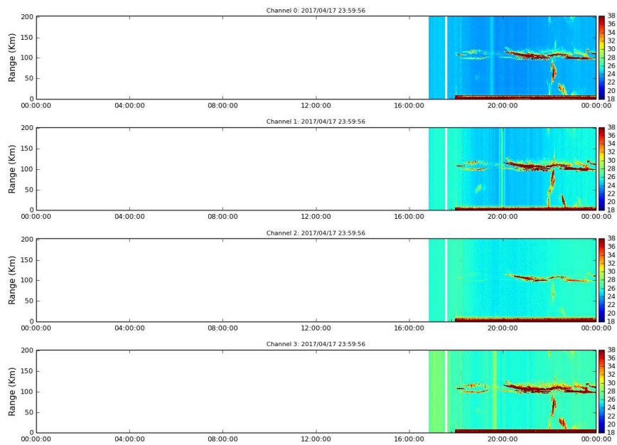
Figure 3. RTI EEJ 2017-04-17.
