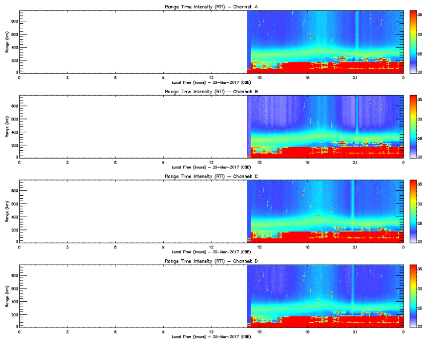
Figure 1.Rti EW_DRIFT 2017-03-29.
