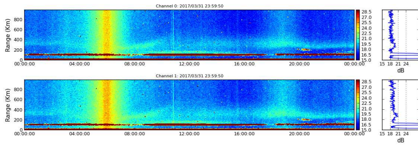
Figure 10. Rti FARADAY 2017-03-31.
