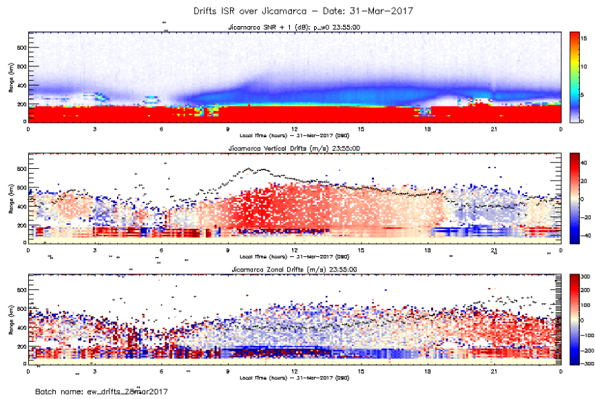
Figure 12. Drifts 2017-03-31.
