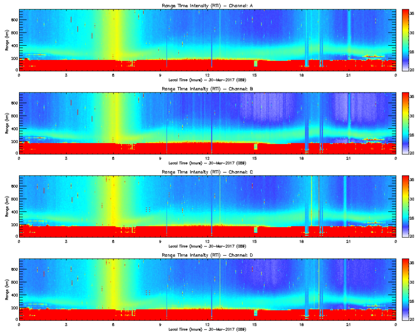
Figure 5. Rti EW_DRIFT 2017-03-30.
