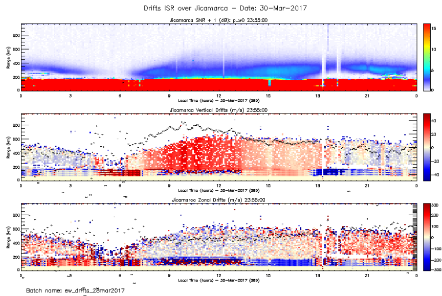
Figure 8. Drifts 2017-03-30.
