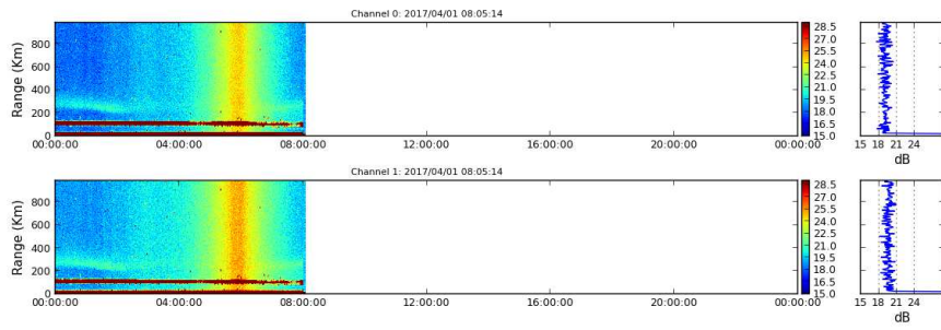
Figure 14. Rti FARADAY 2017-04-01.
