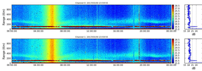
Figure 6. Rti FARADAY 2017-03-30.
