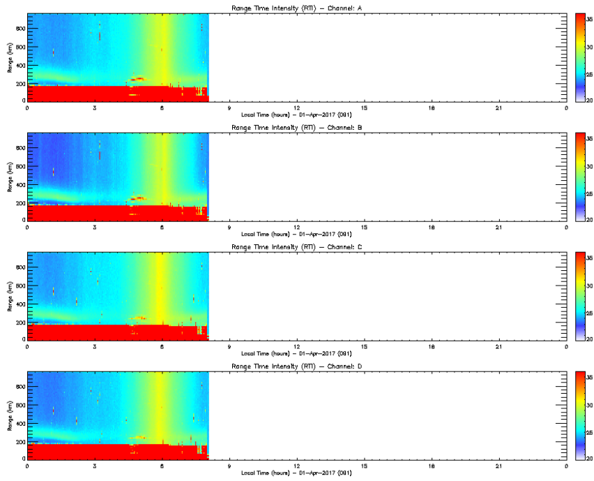
Figure 13. Rti EW_DRIFT 2017-04-01.
