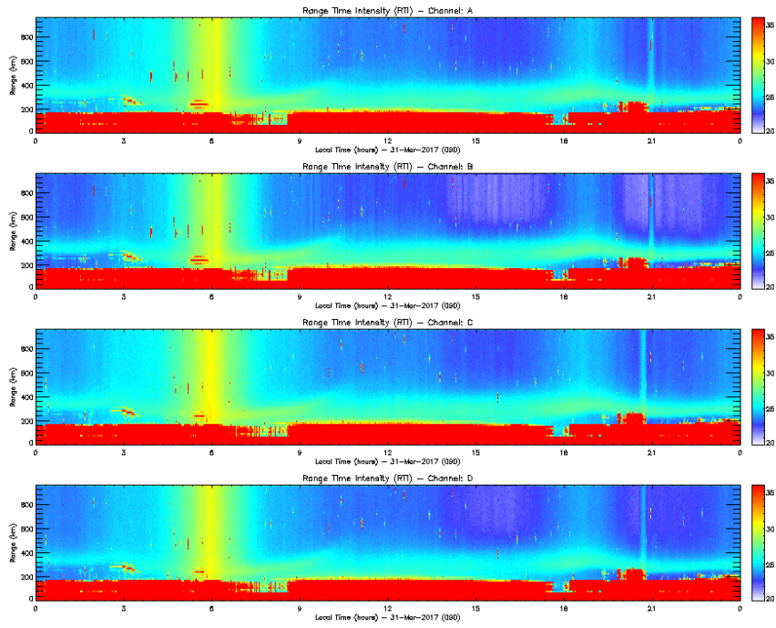
Figure 9. Rti EW_DRIFT 2017-03-31.
