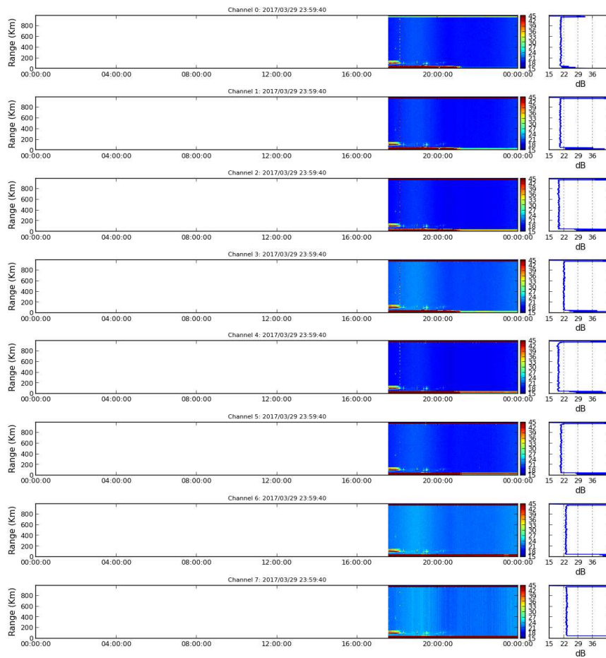
Figure 3. RTI IMAGING 2017-03-29.
