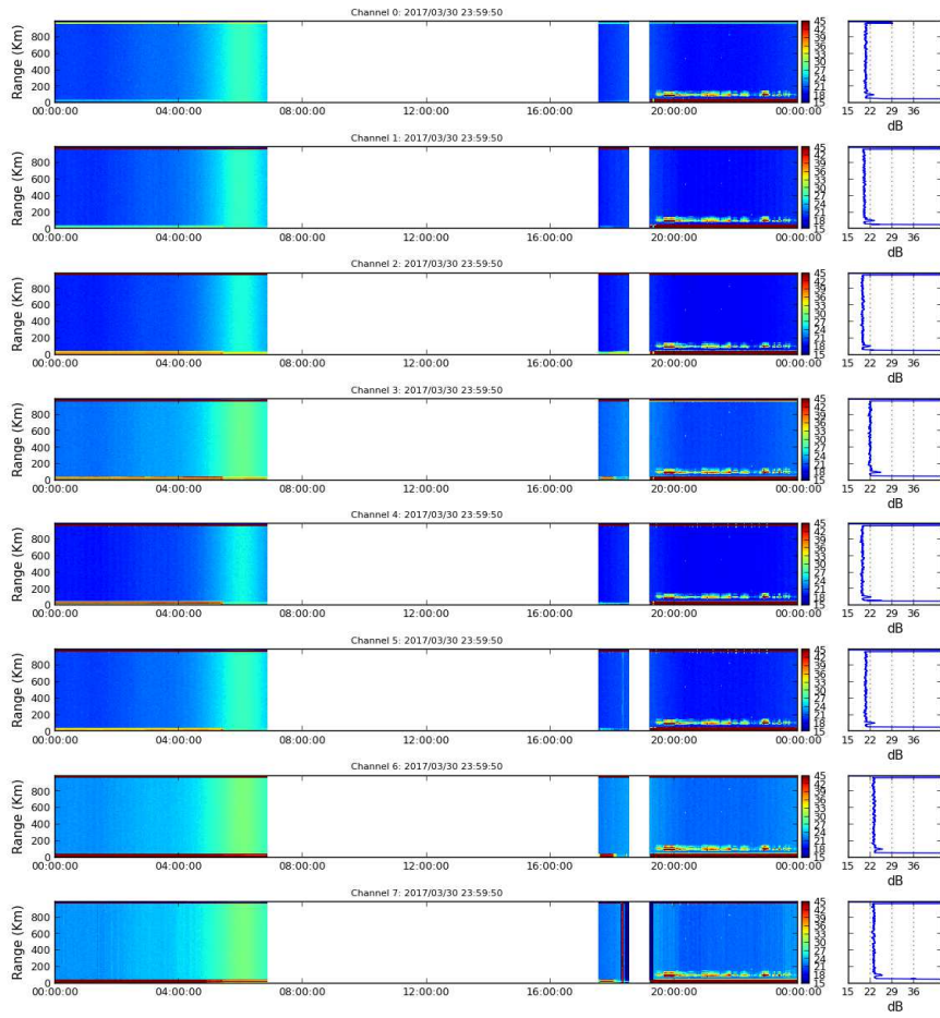
Figure 7. Rti IMAGING 2017-03-30.
