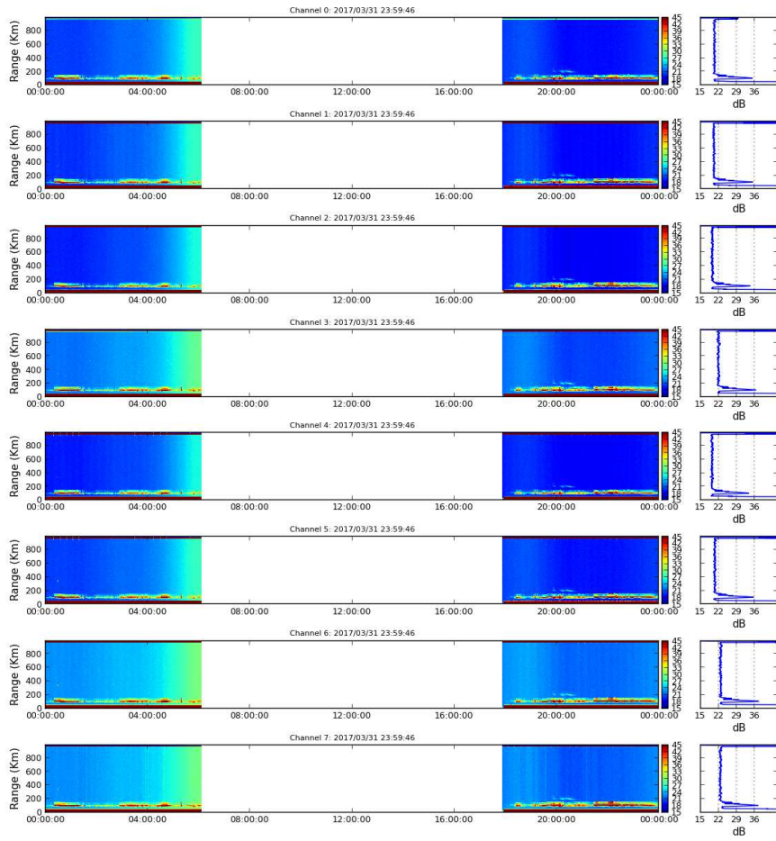
Figure 11. Rti IMAGING 2017-03-31.
