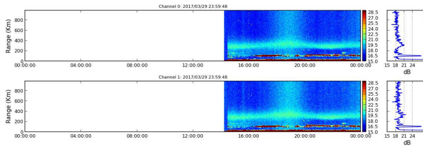
Figure 2. Rti FARADAY 2017-03-29.
