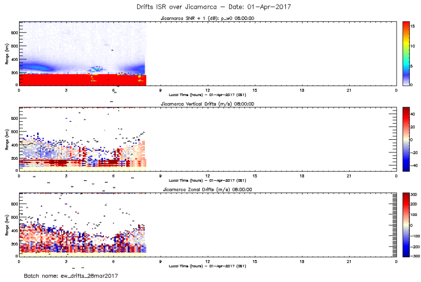
Figure 16. Drifts 2017-04-01.
