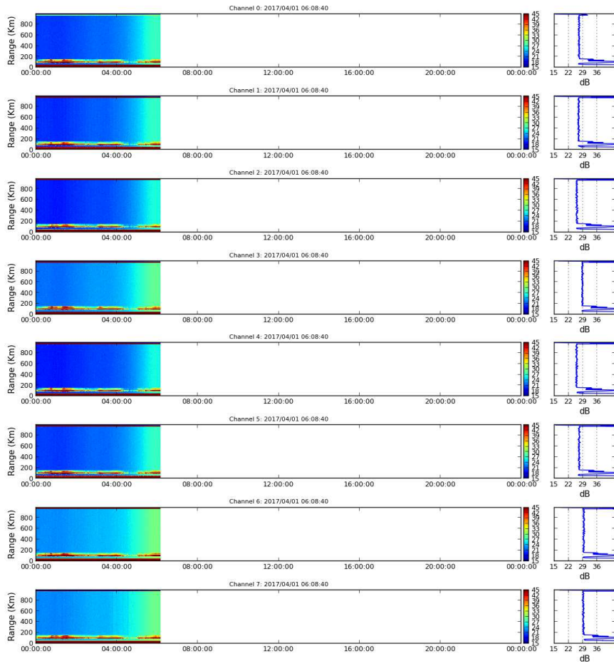
Figure 15. Rti IMAGING 2017-04-01.
