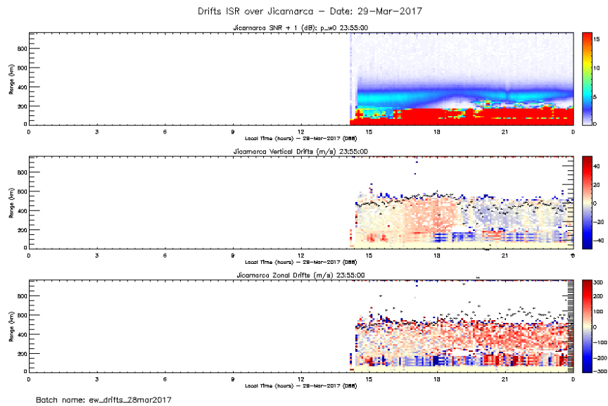
Figure 4. Drifts 2017-03-29.
